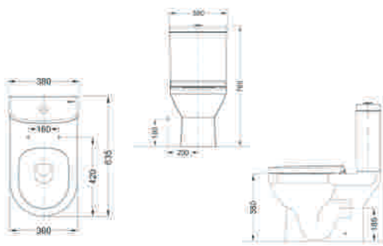
New Moon 2 Pc: C01019XW 635 X 370 X 780 mm
