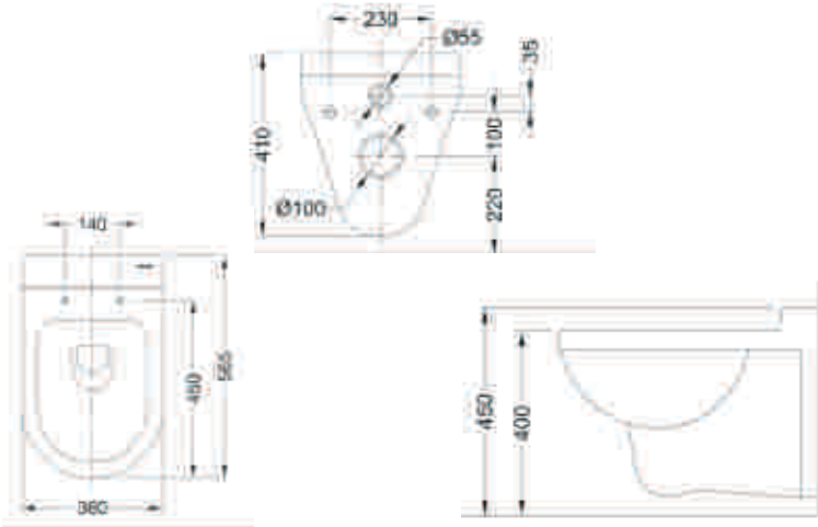
New Moon C2166W 565 X 360 X 410 mm
