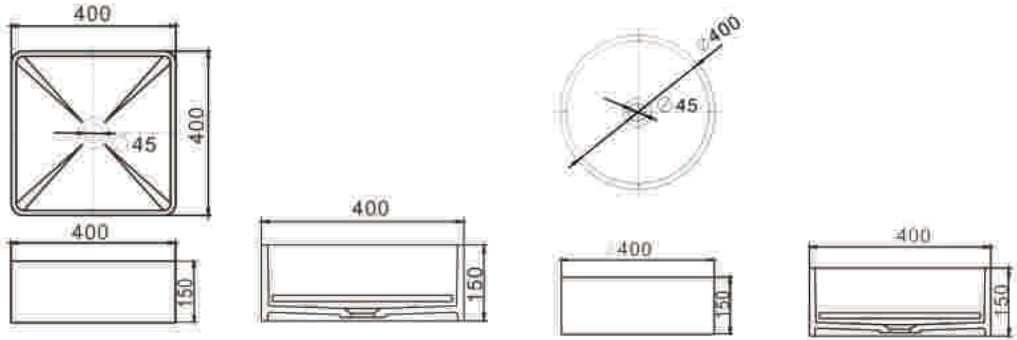
Milano Square Basin C - 3874 - 4 400 X 400 X 150 mm
