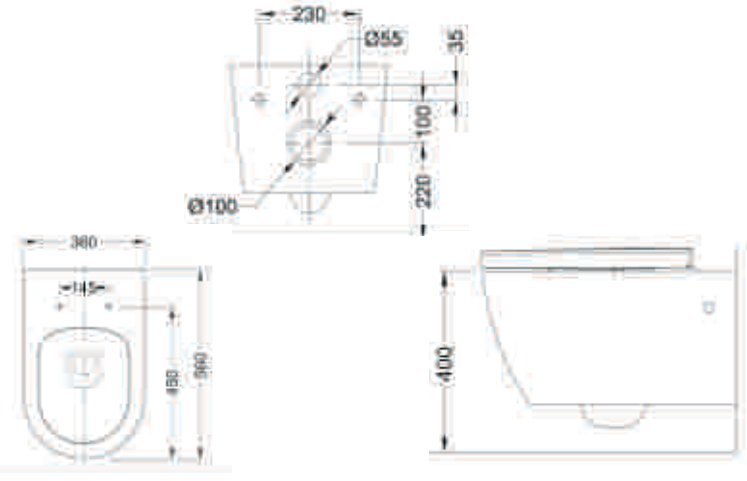
Gina C2190UW 550 X 350 X 360 mm
