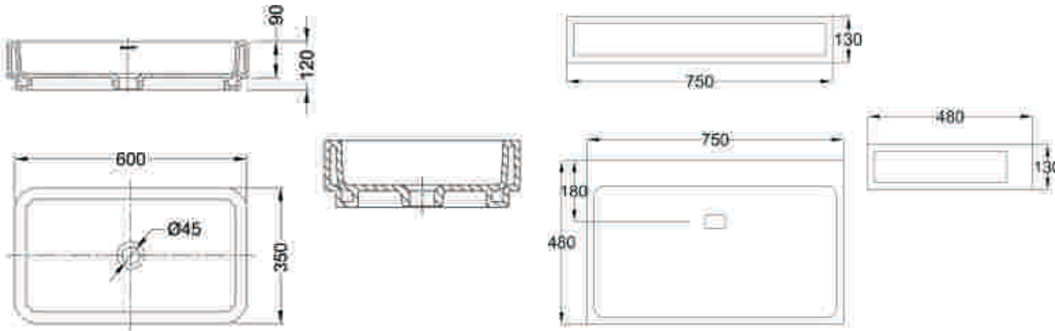
Casa Basin C22144W 600 X 350 X 120 mm
