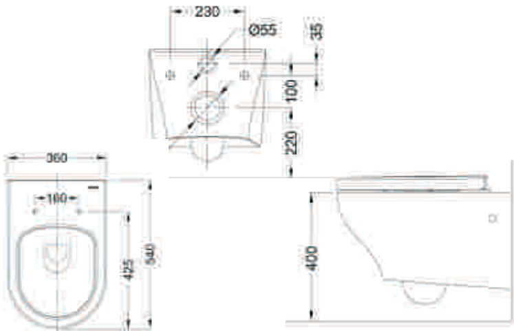
Rael C01017XW 600 X 385 X 160 mm
