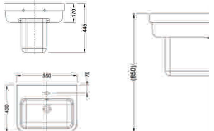
Casa W/H Half Ped. Basin C22133W - I 550 X 430 X 445
