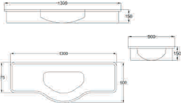
Neo Baroque Basin C22163W-I 1300 X 375 X 150 mm
