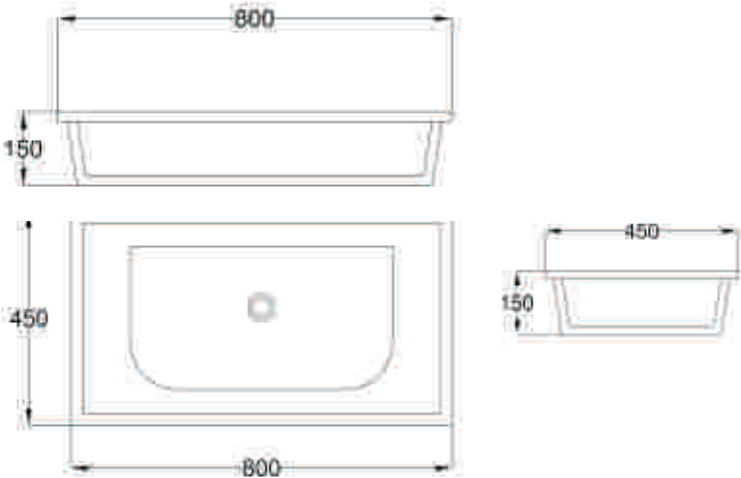
Neo Colonial Basin C22183W-I 800 X 450 X 150 mm
