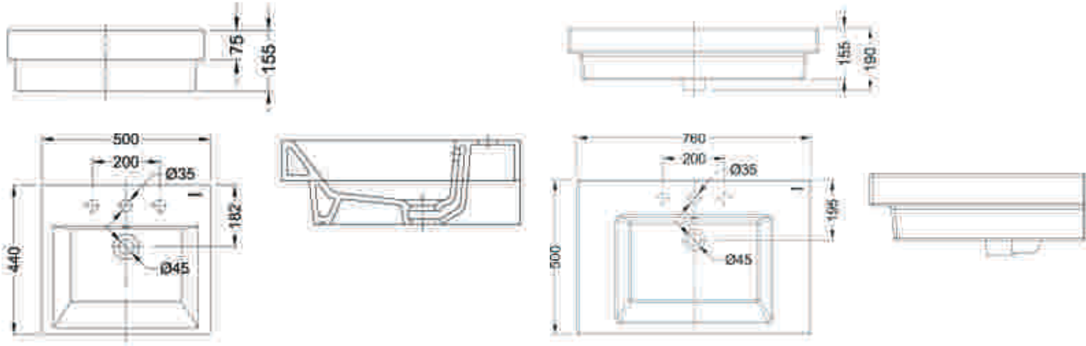
Sharp 50 Basin C22176W - I 500 X 430 X 155 mm
