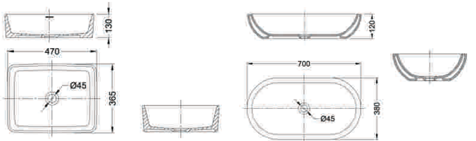
Glacier 47 Basin C2293W 470 X 370 X 125 mm
