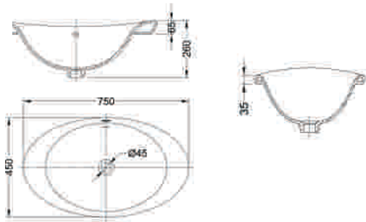
Wave 75 Basin C22142W 750 X 450 X 250 mm
