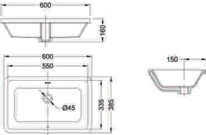
Glacier U/C Basin C22171W 600 X 385 X 160 mm
