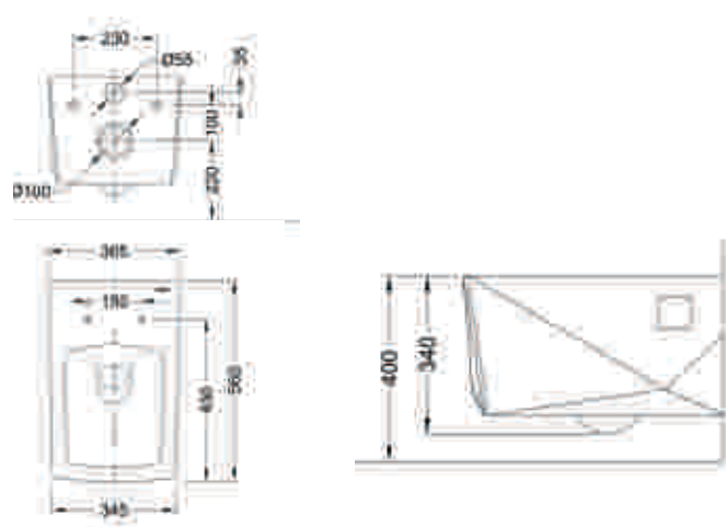
Diamond C2196W 560 X 365 X 340 mm
