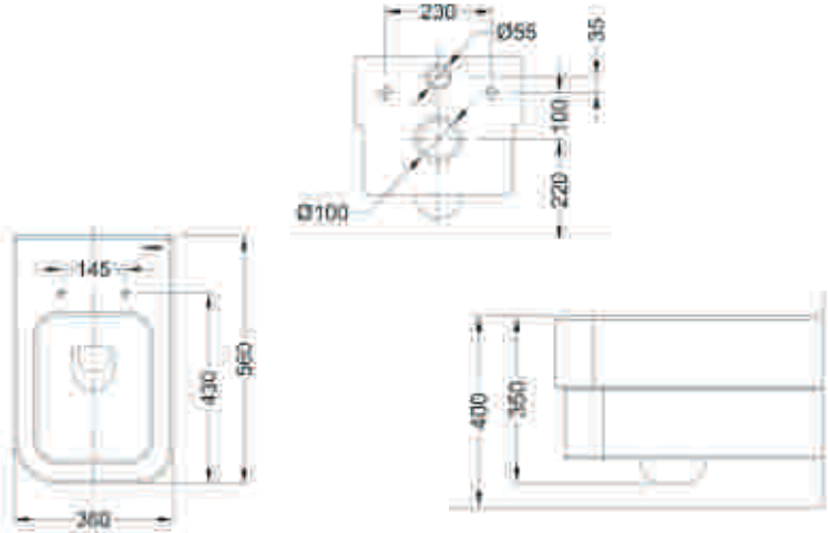
Casa C2160UW 560 X 360 X 330 mm
