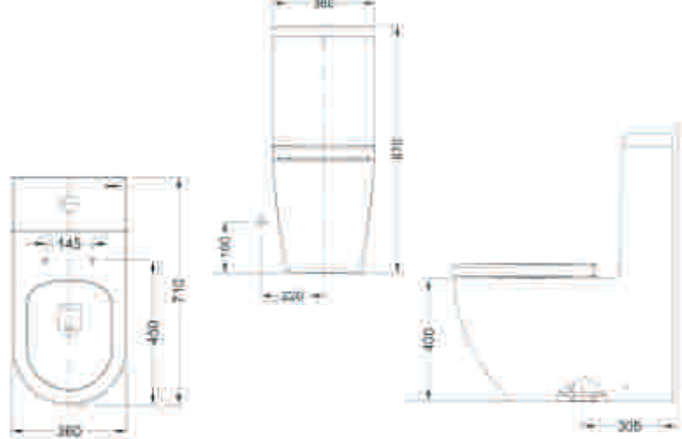
Gina I Pc: C02005W - 3 710 X 360 X 870 mm
