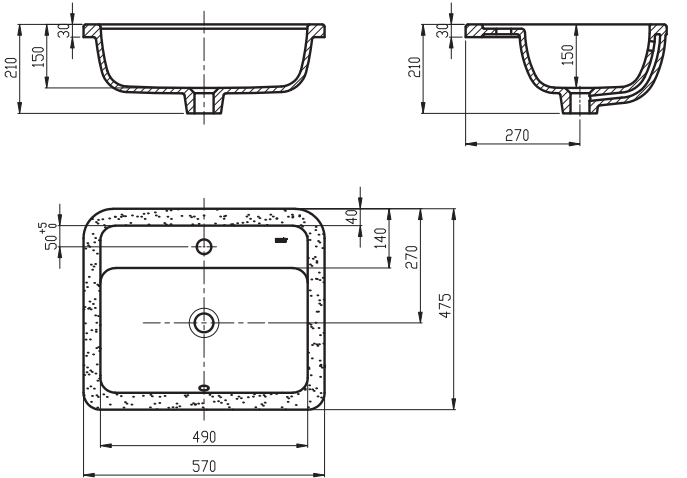
Casa U/C Basin C22145W - I 570 X 475 X 210 mm
