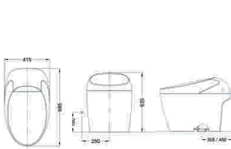
Intelligent Toilet C21118W - 3 685 X 415 X 535 mm
