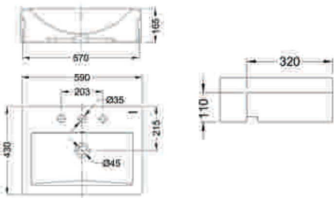
Sharp 59 Semi Recessed Basin C22108W 590 X 430 X 165 mm
