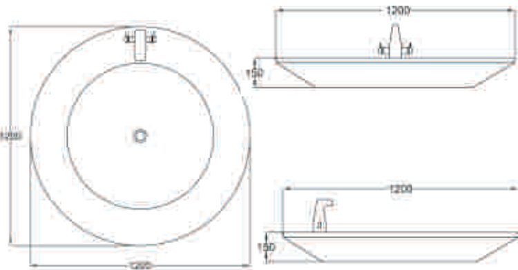
Parisian Basin C2206W-I D1200 X 150 mm
