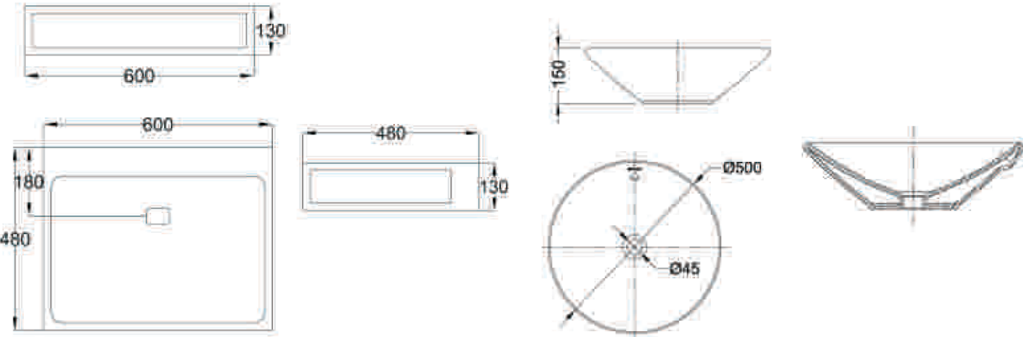
Philis 60 Basin C22192W - IA 600 X 480 X 130 mm
