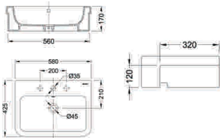
Casa 58 Semi Recessed Basin C22149W 580 X 420 X 170
