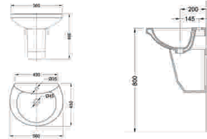
New Moon W/H Half Ped. Basin C22175W - I
