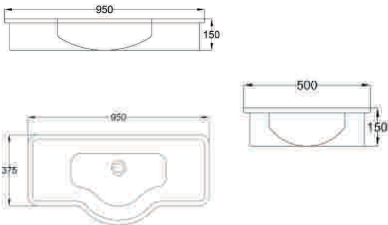
Louis XIV Basin C22182W-I 950 X 375 X 150 mm
