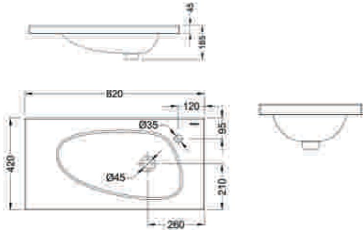
Triangle 82 Basin C2273W - I 820 X 420 X 185 mm
